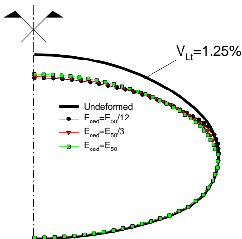
Figure 5. Tunnel-deformed shape for the different cases.
